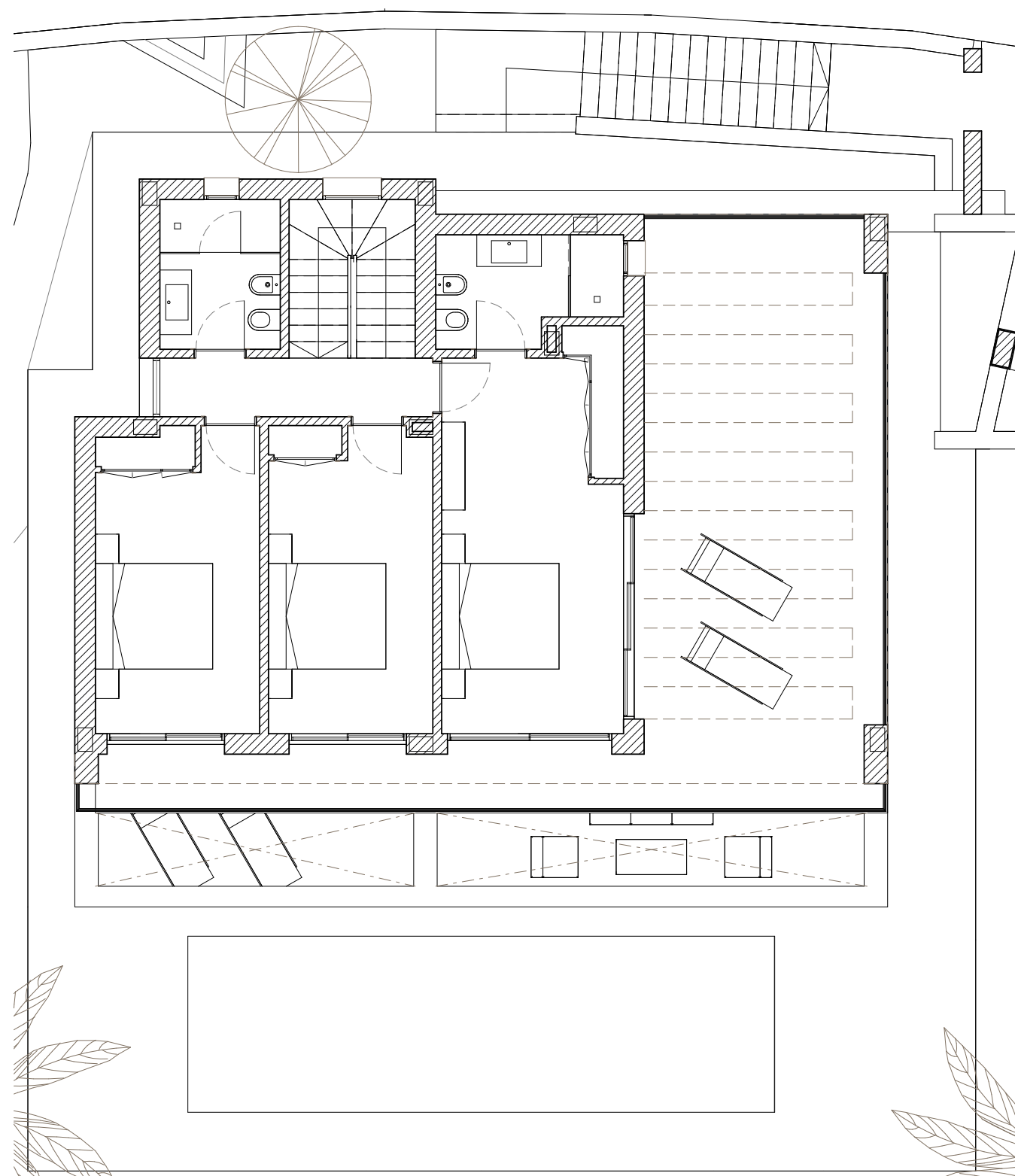
FIRST FLOOR
